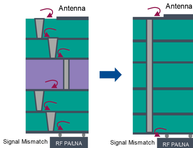
Figure 7: Optimized substrate stack-up and RDL/via routing can improve antenna performance by reducing signal mismatch.
